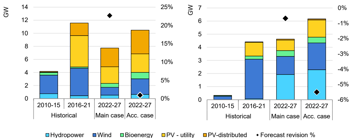
Figure 1.35 Mexico renewable capacity additions, 2010-2027 (left) and Argentina renewable capacity additions, 2010-2027 (right)
