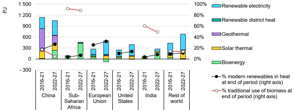
Figure 3.4 Buildings sector increase in renewable heat consumption and share of renewables in heat demand, selected regions, 2016-2027
