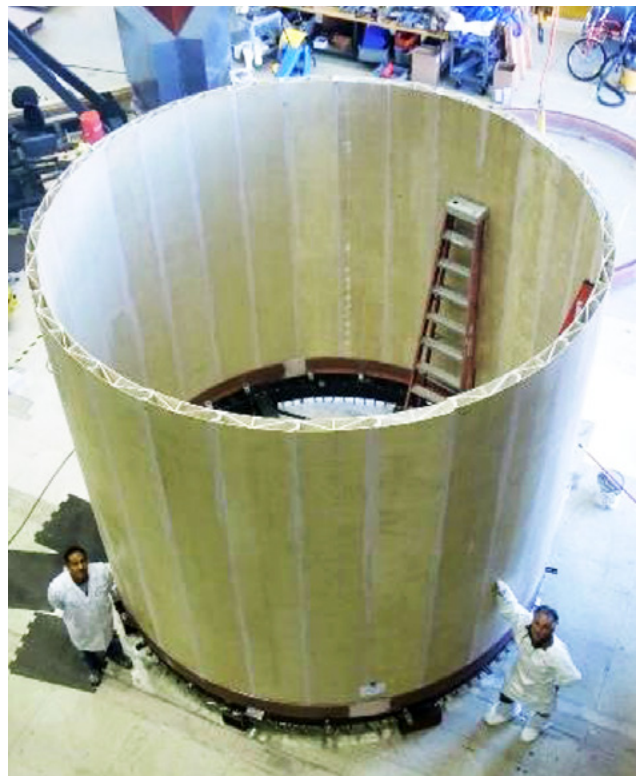
Figure 8.2 Lockheed Martin’s CWP R&D programme with a 4 m pipe next to two engineers
