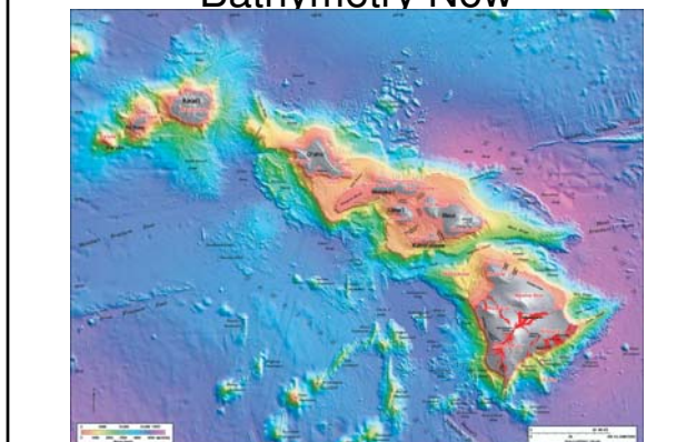
Bathymetry Now
